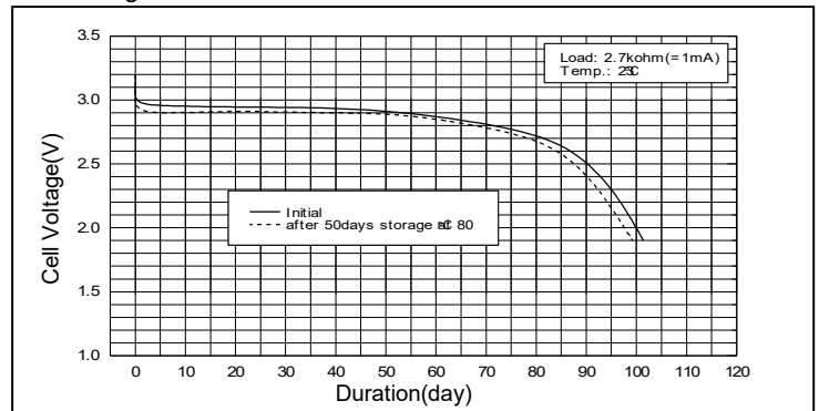
Discharge Characteristics of CR17450SE
