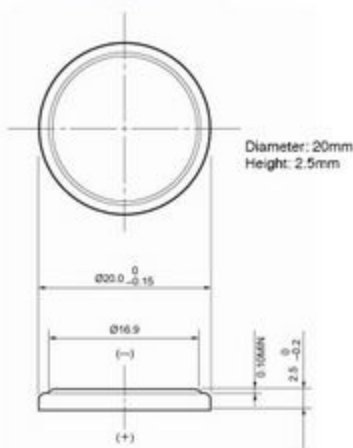
Dimension Drawing
