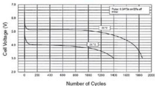
Pulse Discharge Characteristics of 2CR5
