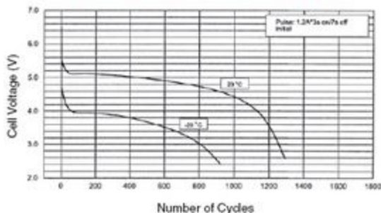
Pulse Discharge Characteristics of 2CR5
