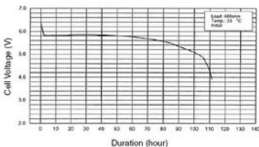
Discharge Characteristics of 2CR5
